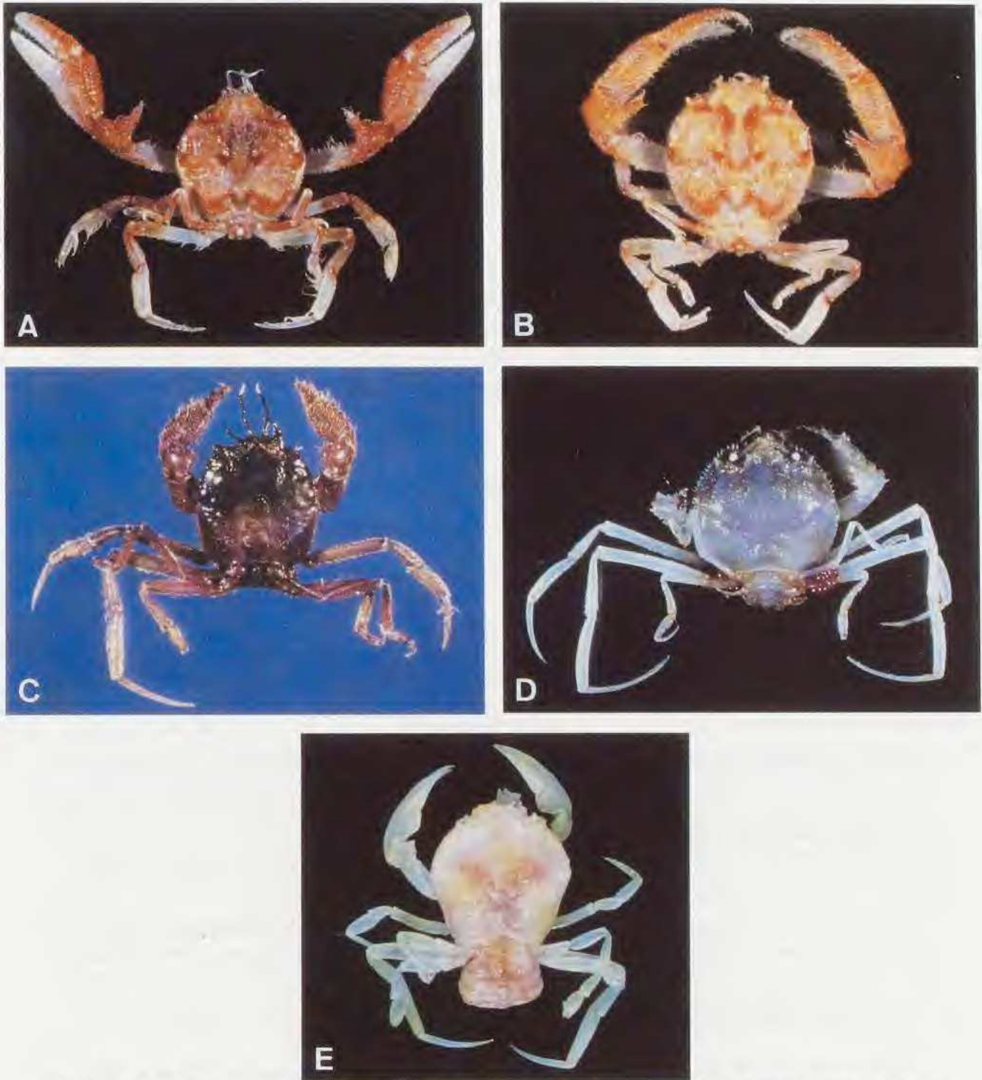
FIG. 4. — A-B, Xeinnostoma richeri Tavares, 1993 : A, ♂, Vanuatu, MUSORSTOM 8, st. CP 1024, 17°48'S, 168°39'E, 335-370 m; B, ♂, Nouvelle-Calédonie, SMIB 8, st. DW 165, 24°47'S, 168°03'E, 372-660 m. — C, Ketamia limatula Tavares, 1993, ♂, Vanuatu, MUSORSTOM 8, st. CP 1001, 18°49'S, 168°59'E, 150-250 m. — D, Krangalangia spinosa (Zarenkov, 1970), ♀ ovigère, Vanuatu, MUSORSTOM 8, st. CP 1039, 18°01'S, 168°48'E, 920-950 m. — E, Phyllotymolinum crosnieri Tavares, 1993, ♀ ovigère, Nouvelle-Calédonie, BATHUS 3, st. DW 836, 23°02'S, 166°59'E, 295-306 m.
